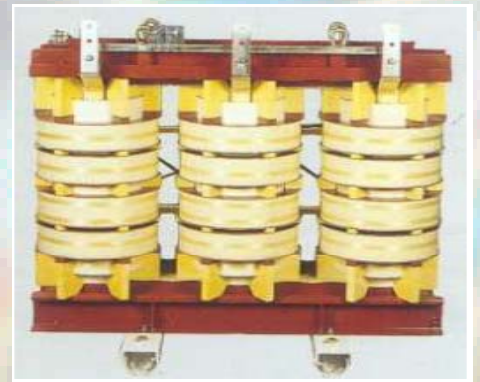
Dry distribution transformer Primary: 20 000V - Secondary: 410V Power: 630 kVA
