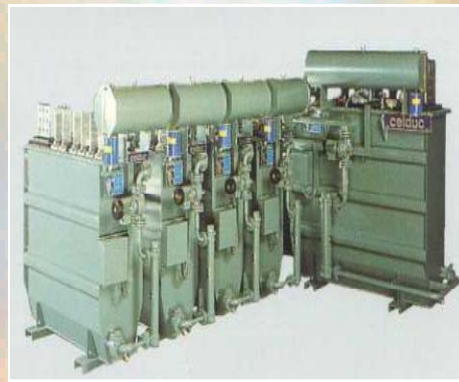
Double secondary windings for converters Primary: 6 000V - Secondary: 42V et 60V Power: 910 kVA et 2 080 kVA
